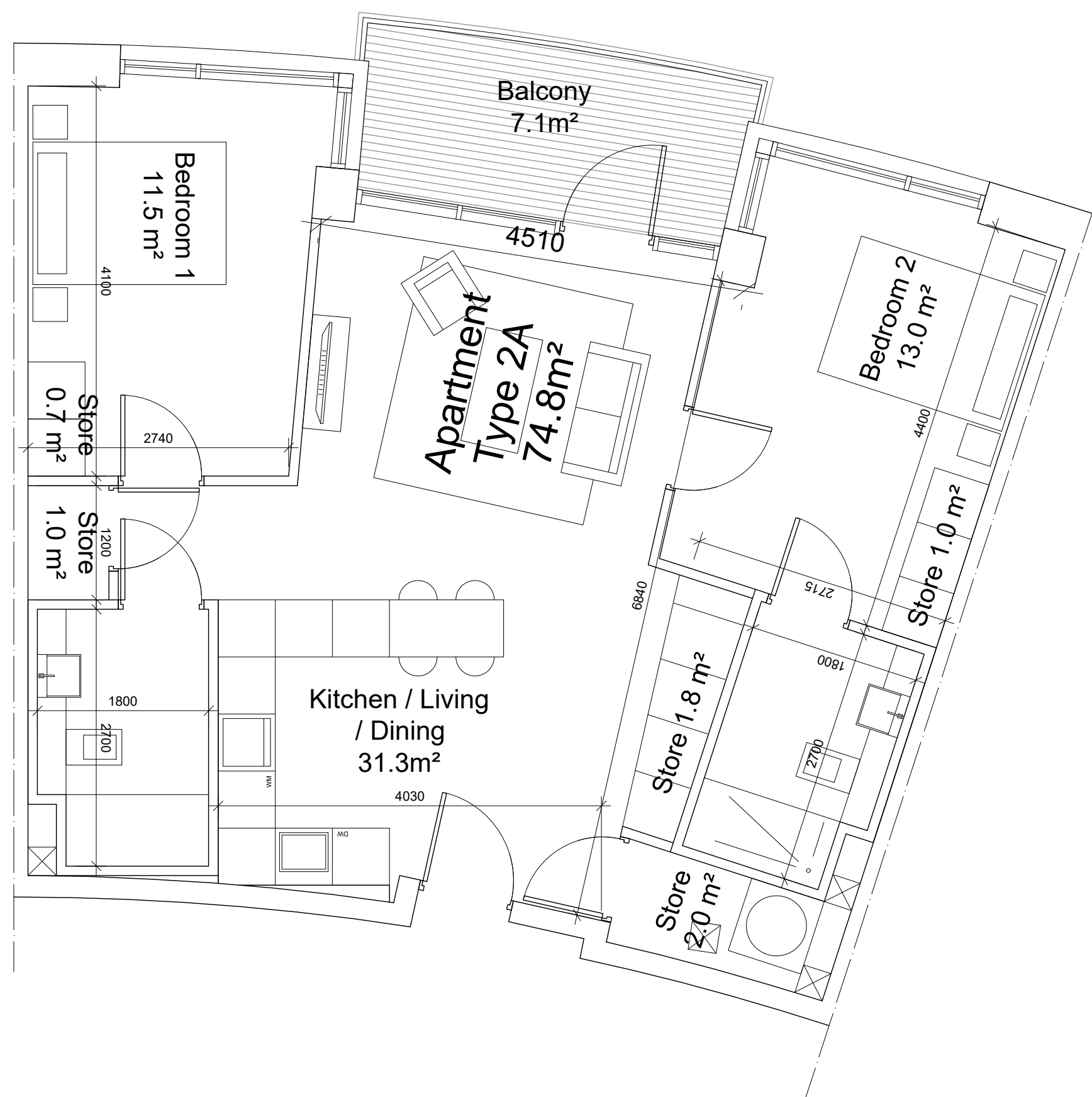
01 2 Bed Apartment - Type 2A (29 Units) SCALE 1:50
