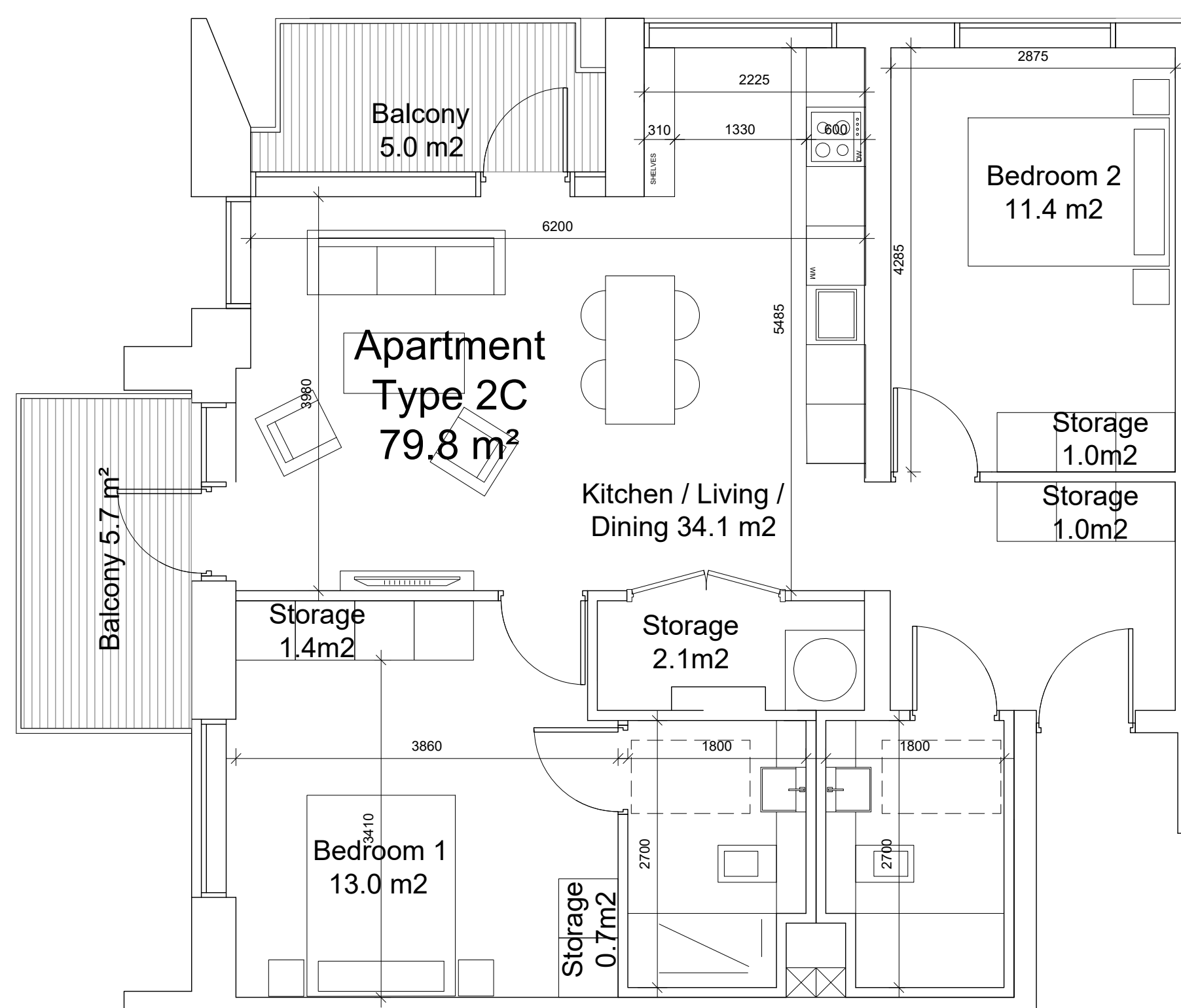
03 2 Bed Apartment - Type 2C (3 units) SCALE 1:50
