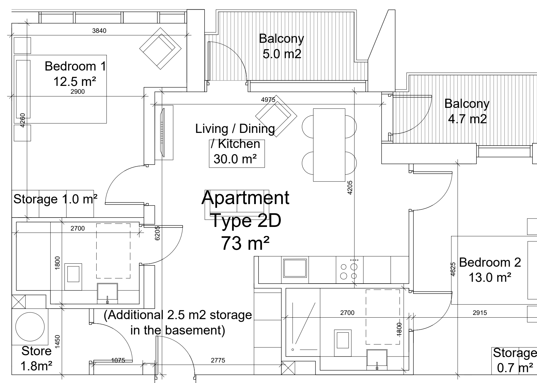
04 2 Bed Apartment - Type 2D (4 Units) SCALE 1:50
